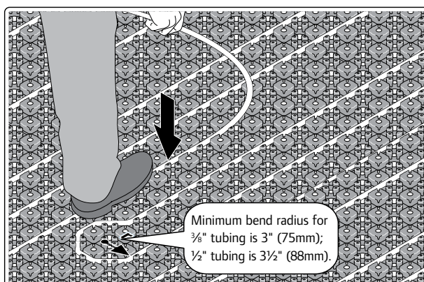
Figure 15: Install Tubing
