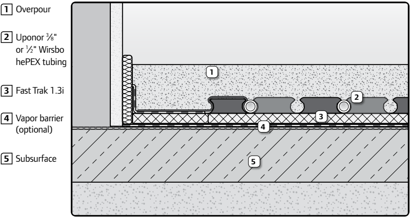
Figure 10: Fast Trak 1.3i Installation Application
