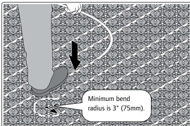
Figure 8: Install Tubing
