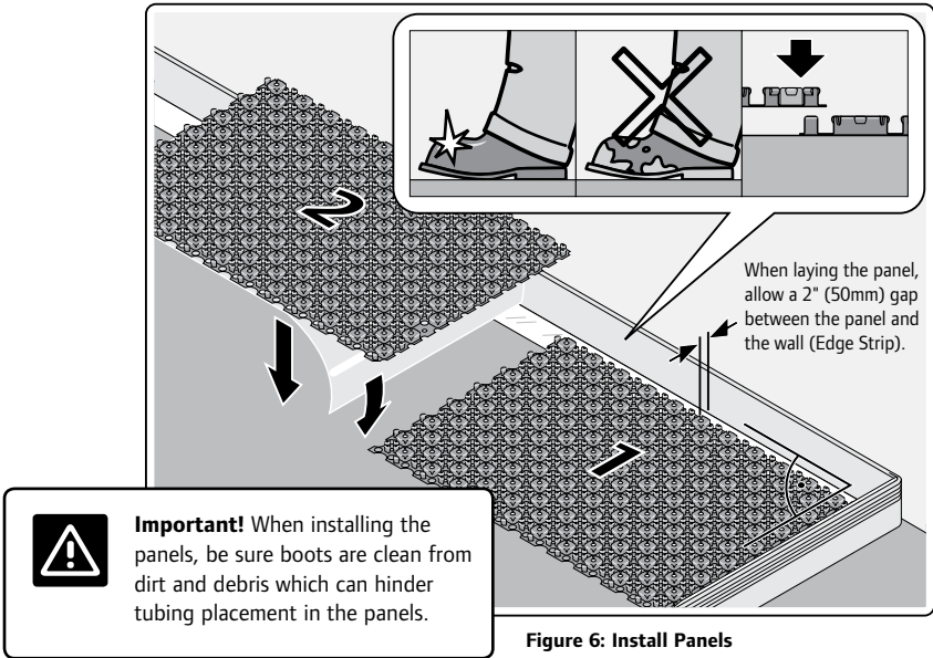
Figure 6: Install Panels
