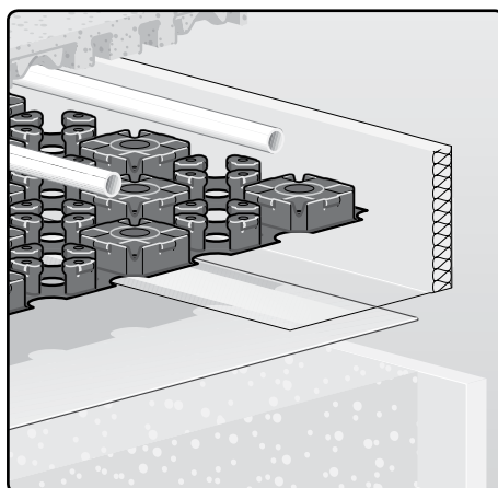
Figure 5: Proper Edge Strip Location
