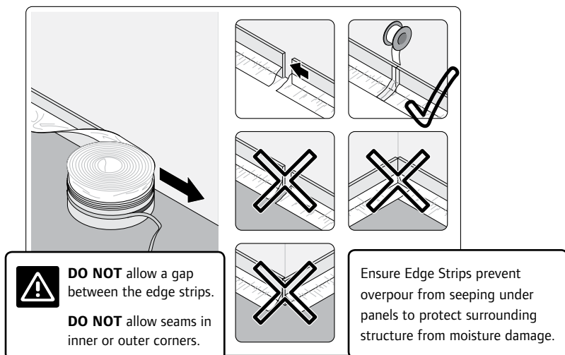
Figure 11: Install Edge Strips
